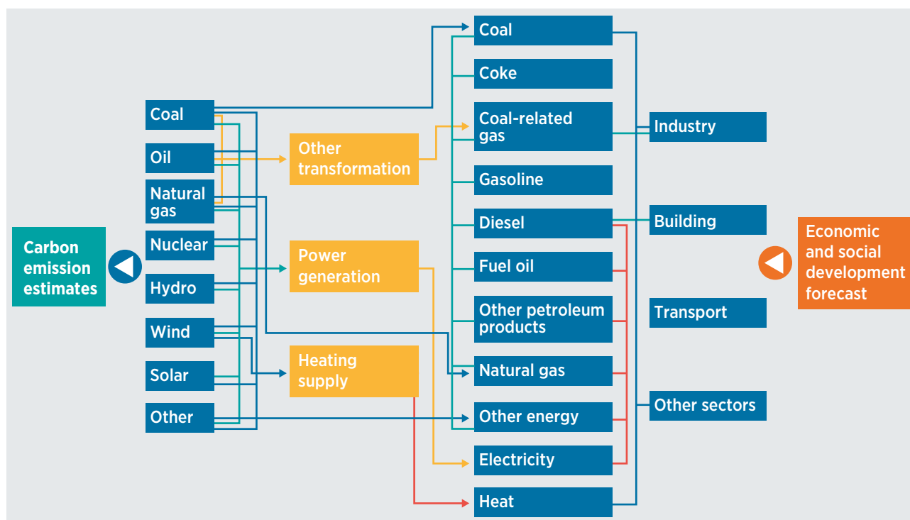
Figure 45 Integrated model: China's economy - energy - environment
