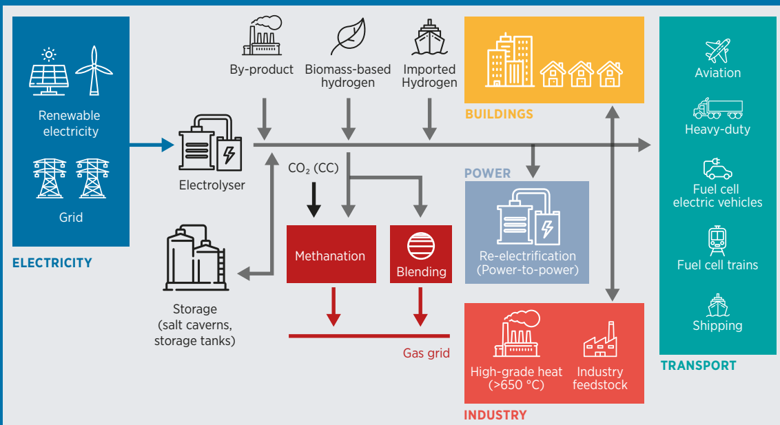
Figure 10 Integration of VRE into end uses by means of hydrogen
