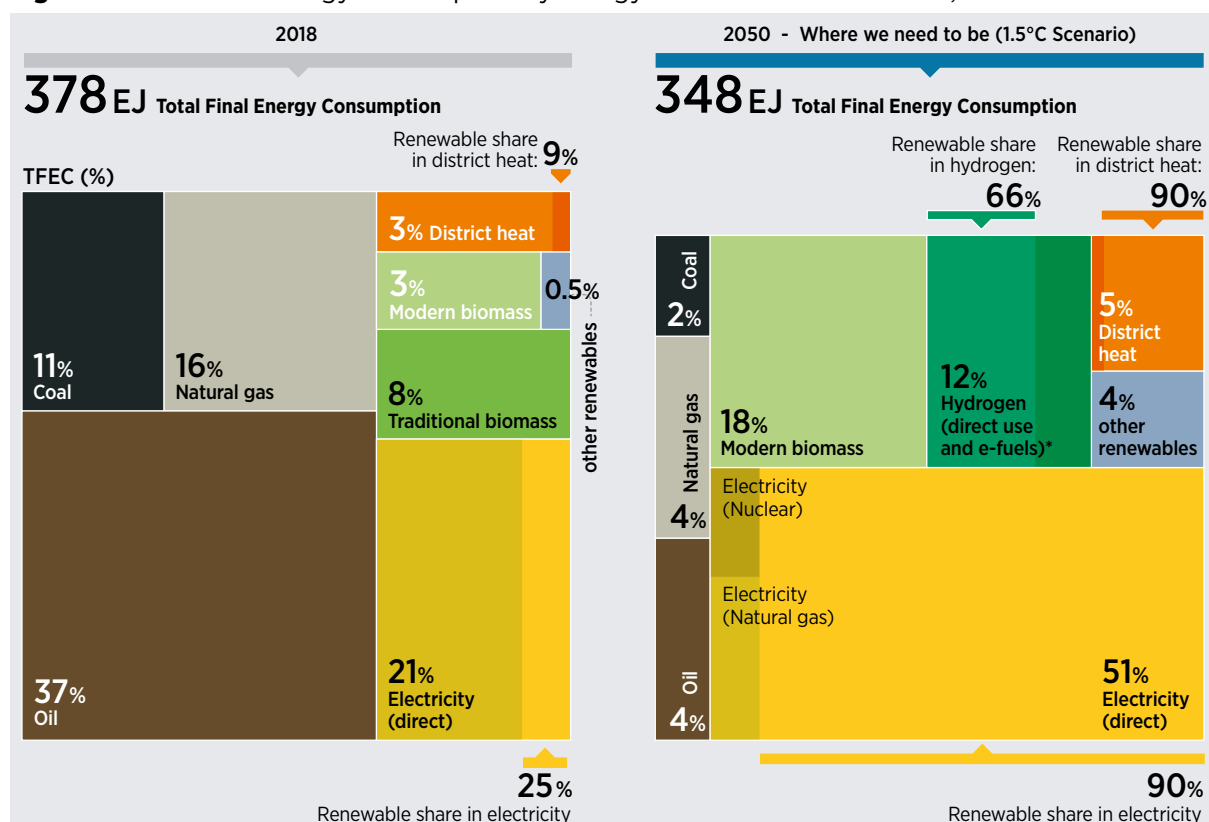
Figure 23 Total final energy consumption by energy carrier in 2017 in the TES, 2050
