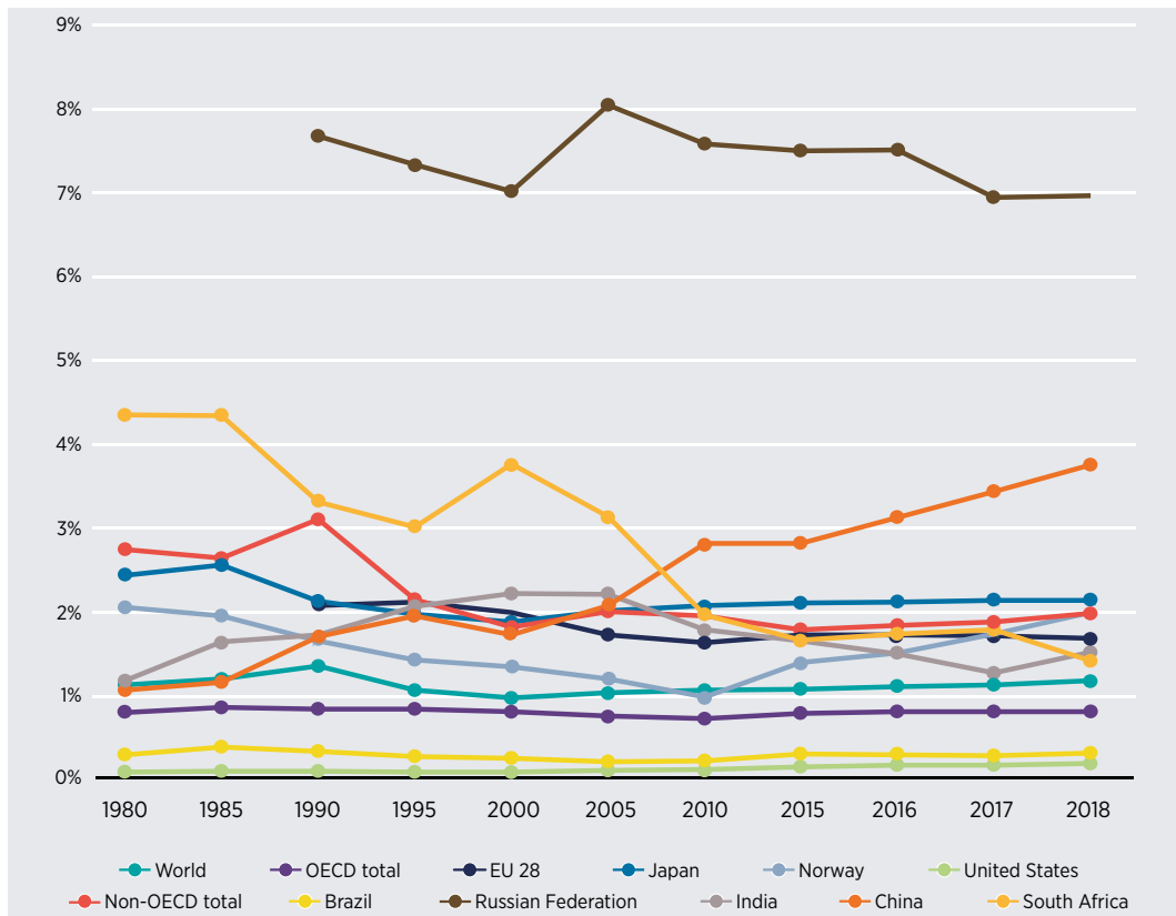
Figure 40 The level of electrification of transportation in selected countries during 1980-2018 (IEA, 2020a)
