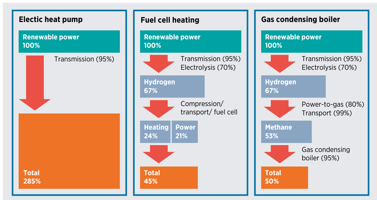
Figure 17 Efficiencies for different heating systems, starting from renewable electricity
