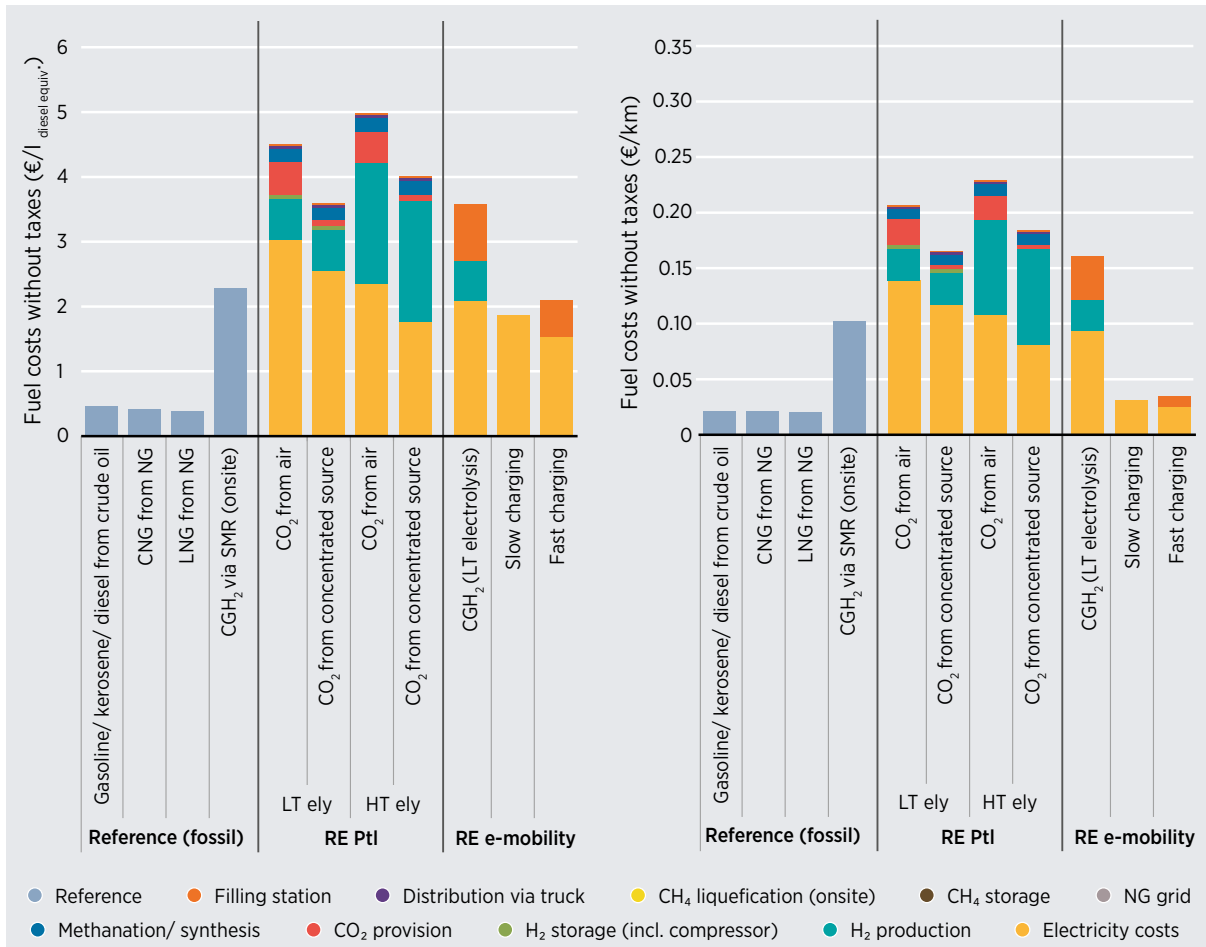
Figure 8 Transport fuel costs: well-to-tank per unit of fuel volume (left) and well-to-wheel per unit of distance (right)
