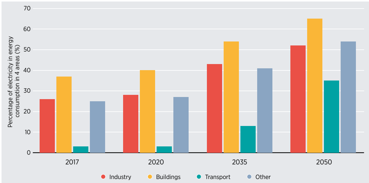
Figure 28 Electrification rate of various sectors in the Electrification Scenario
