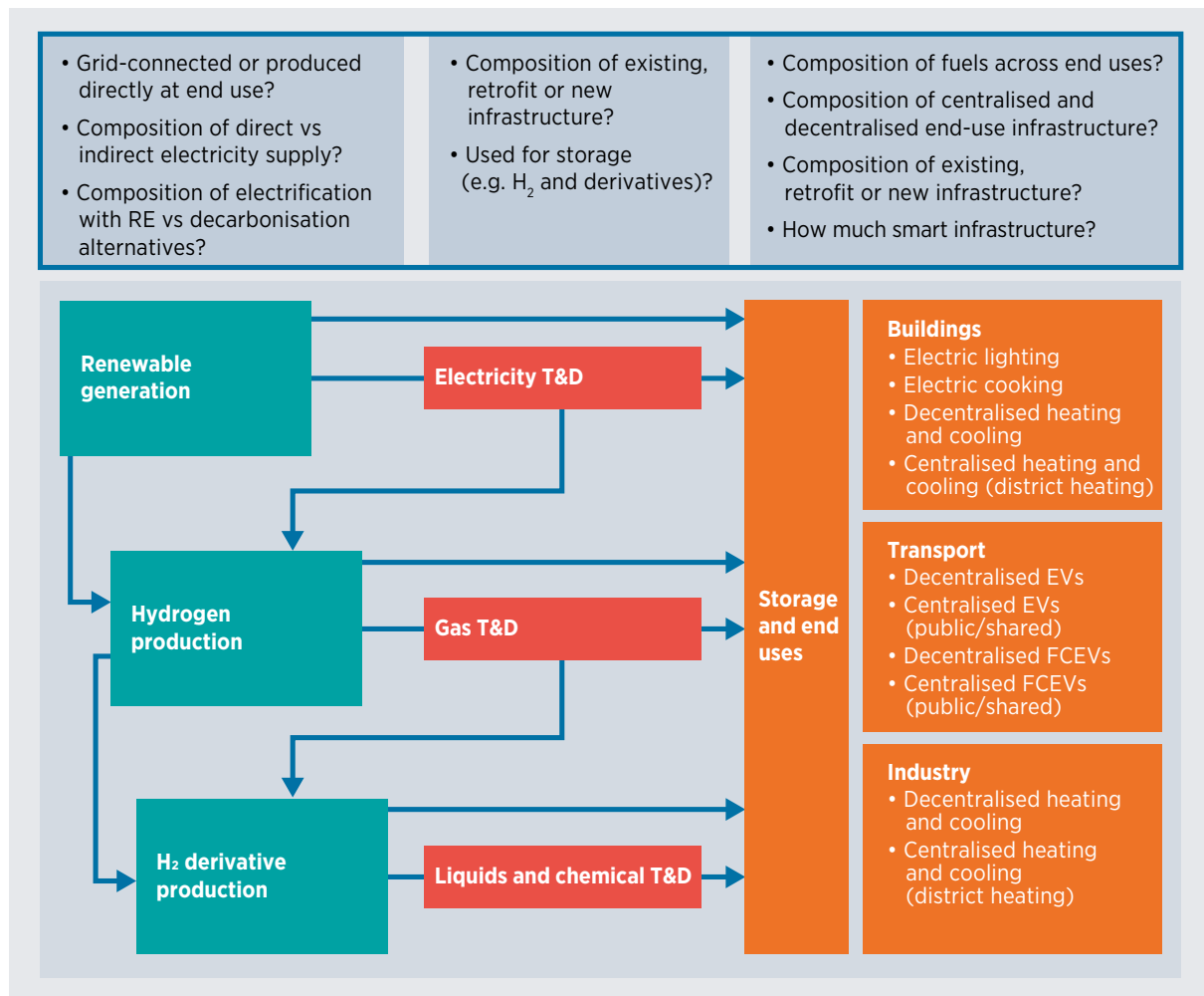
Figure 18 Overall infrastructure landscape for smart electrification pathways
