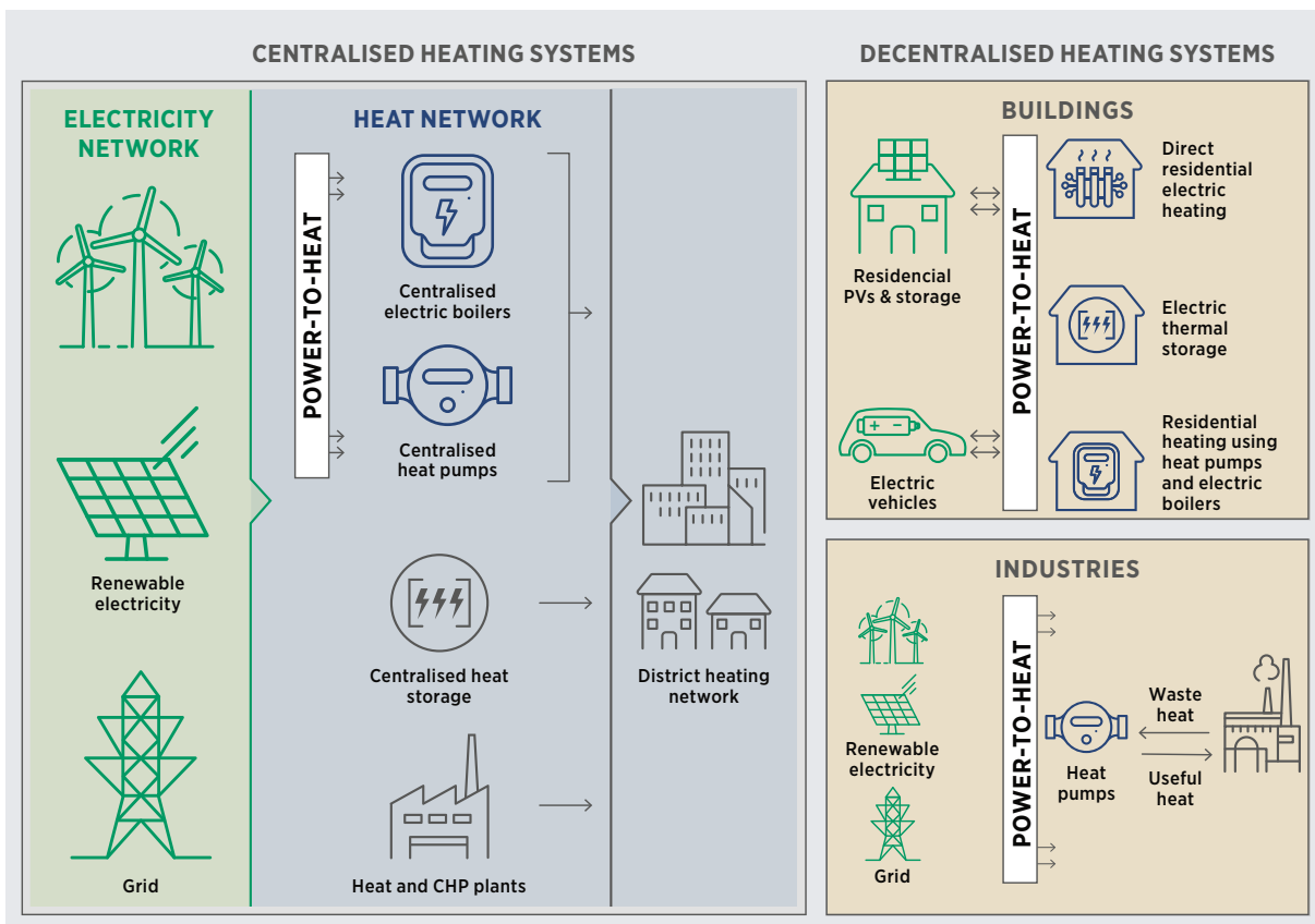
Figure 14 Types of heating systems that use electricity
