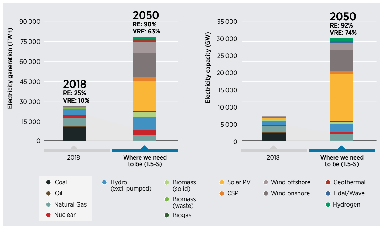
Figure 22 Electricity generation mix (TWh) and power generation installed capacity (GW) by fuel, 2018 actual and 2050 1.5°C Scenario
