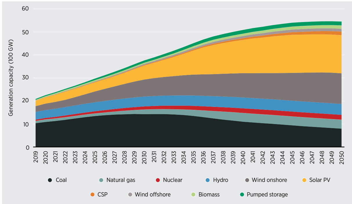
Figure 30 Generation capacity of various power sources in the Electrification Scenario, 2019-2050
