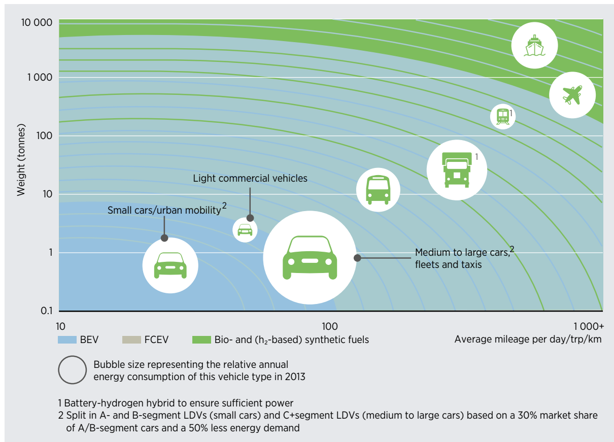
Figure 5 Segmentation of the transport market
