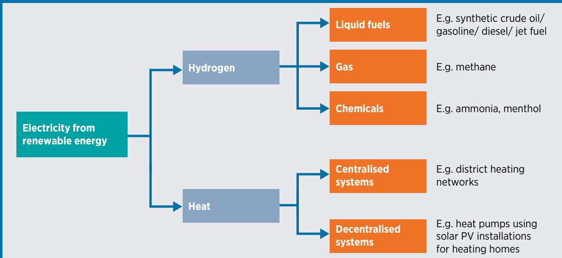
Figure 9 Classification of Power-to-X technologies
