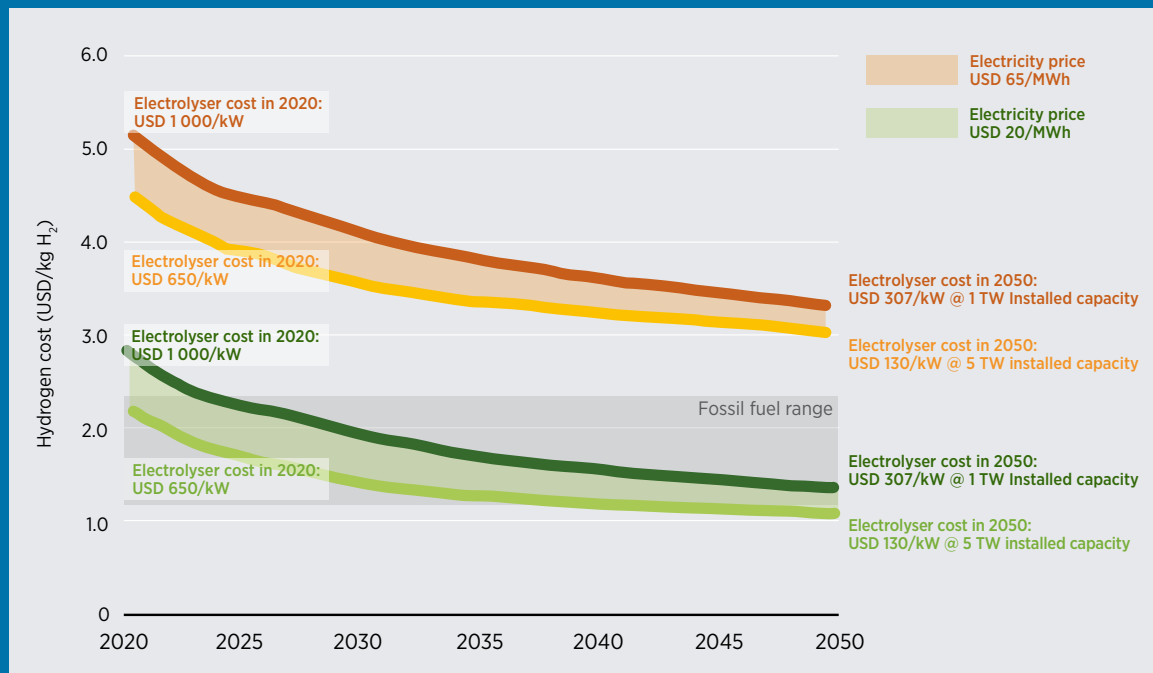
Figure 11 Cost of green hydrogen production as a function of electrolyser deployment
