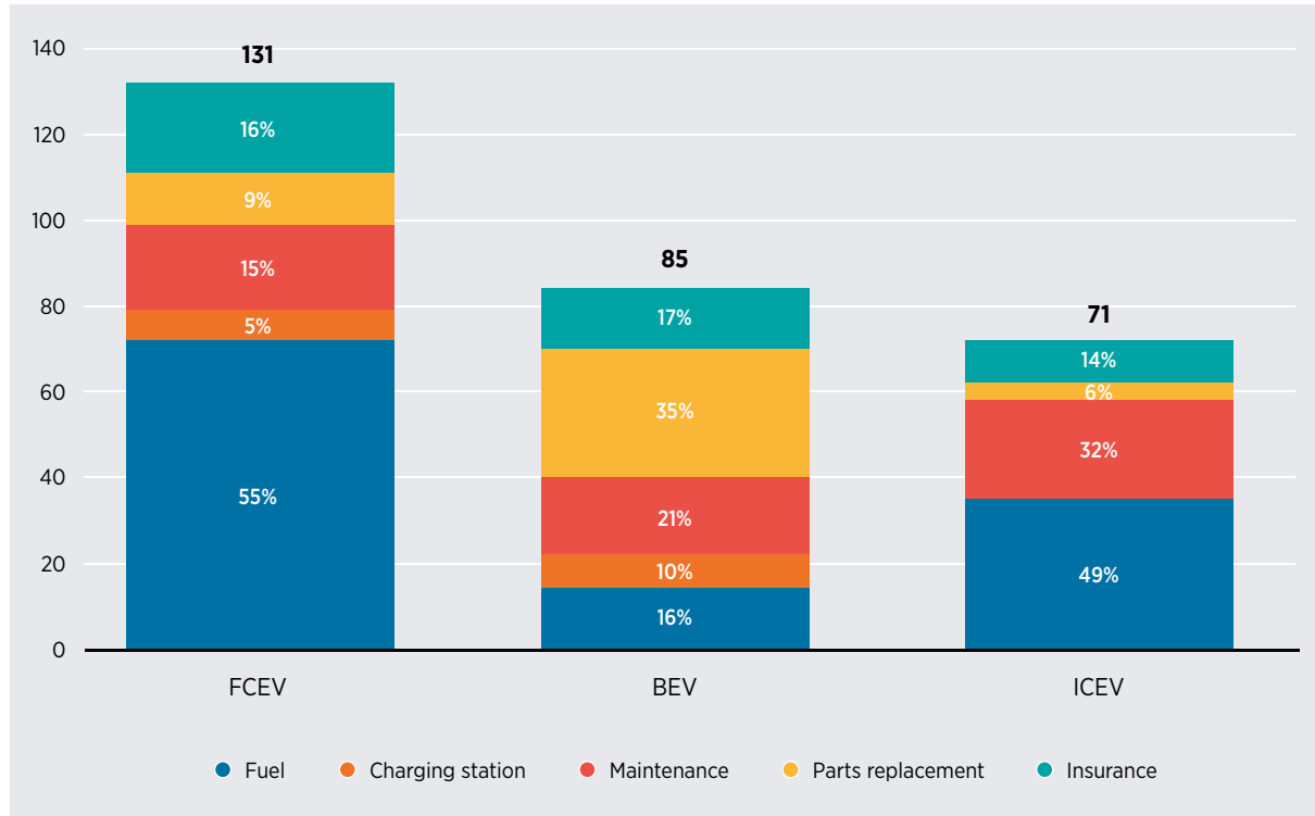
Figure 7 Breakdown of bus operational cost (USD 000/100 km)
