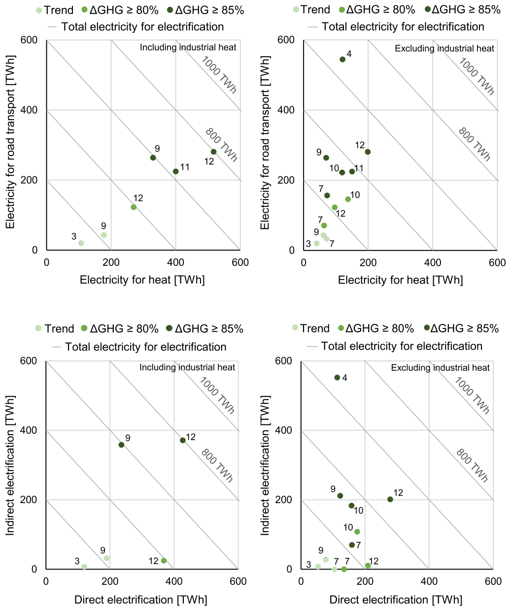
Figure 19 Levels of electrification in a sensitivity analysis of future German transport and heat sector scenarios
