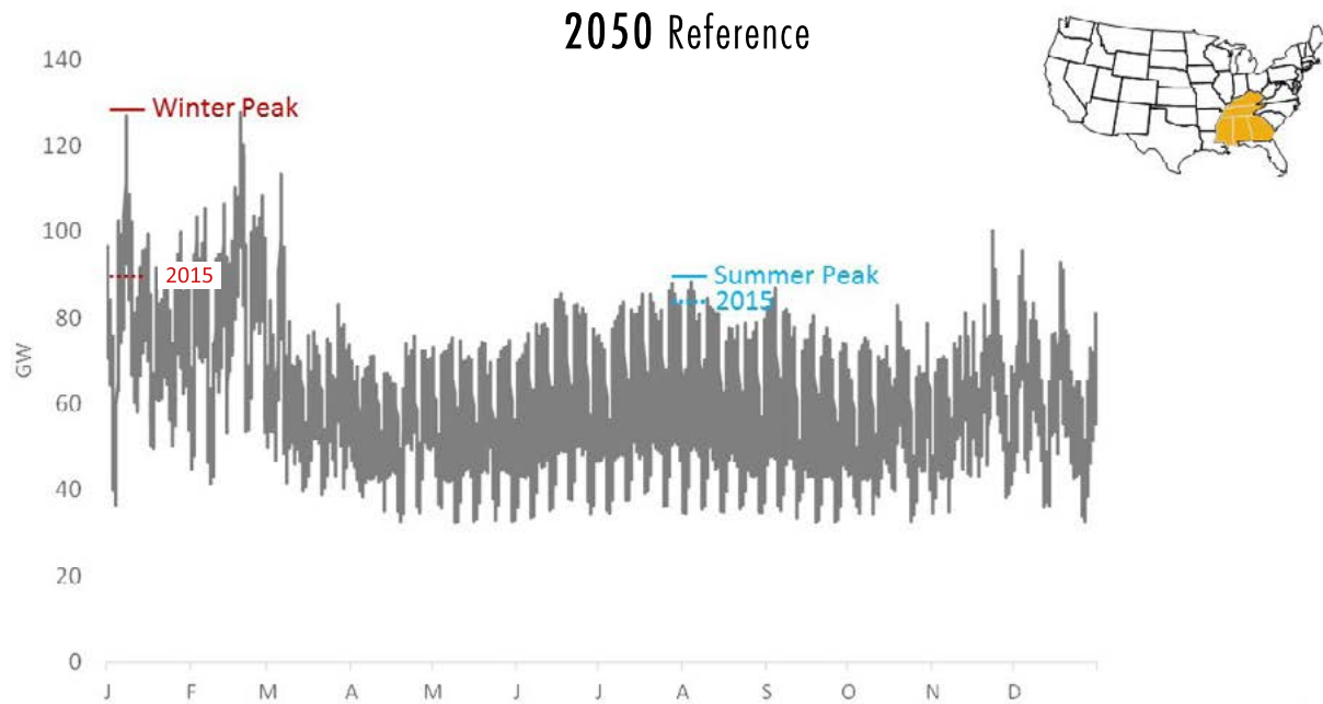
Figure 15 Electricity demand in EPRI 2050 Reference scenario for the Southeast United States
